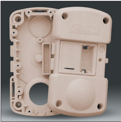
Z Corp. model (top) and actual product (right) of a Job Site Security Sensor Housing
